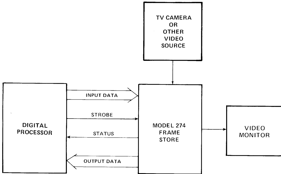
TYPICAL FRAME STORE/DIGITAL PROCESSOR SYSTEM
