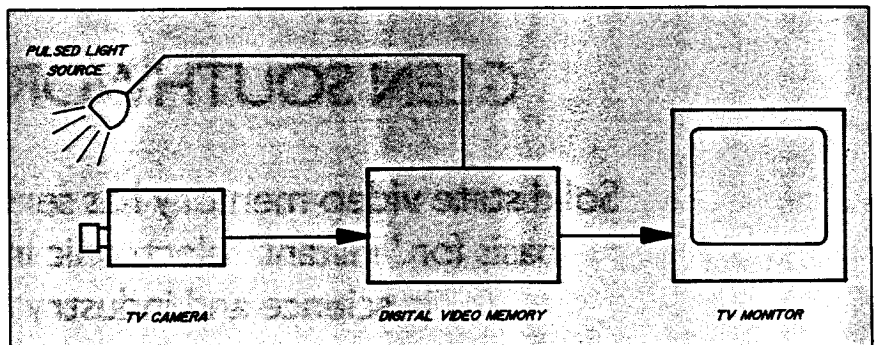
Figure 1. Block diagram of typical digital video memory set-up.
